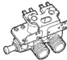
120V Water Valve 3/8" & 1/2" adapter Reference: 5303207418 5308006679
